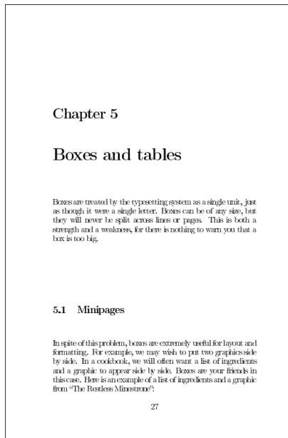
Figure 9.1: Default layout
